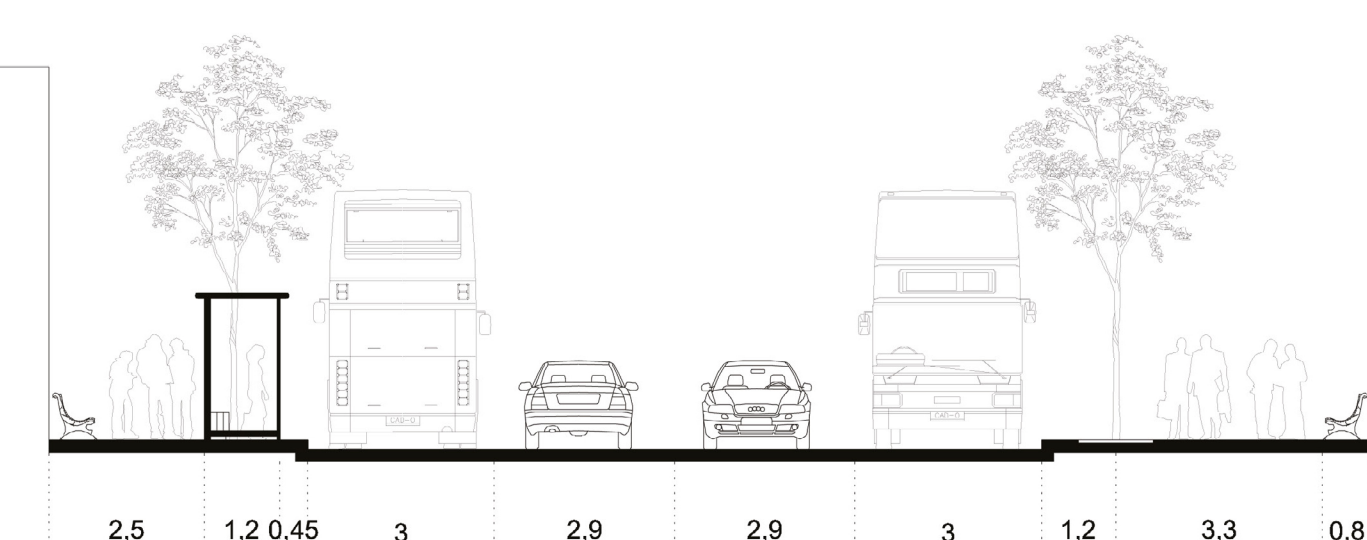
Section 2-2
