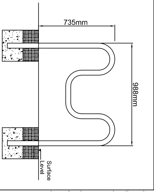
INSET A DETAILS OF 'M' SHAPED CYCLE STAND
