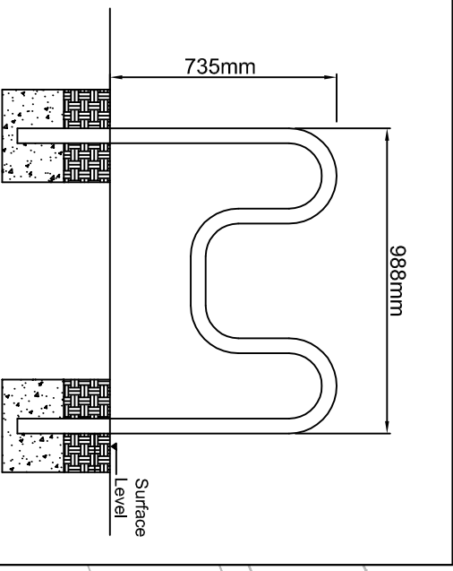
INSET A DETAILS OF 'W' SHAPED CYCLE STAND
