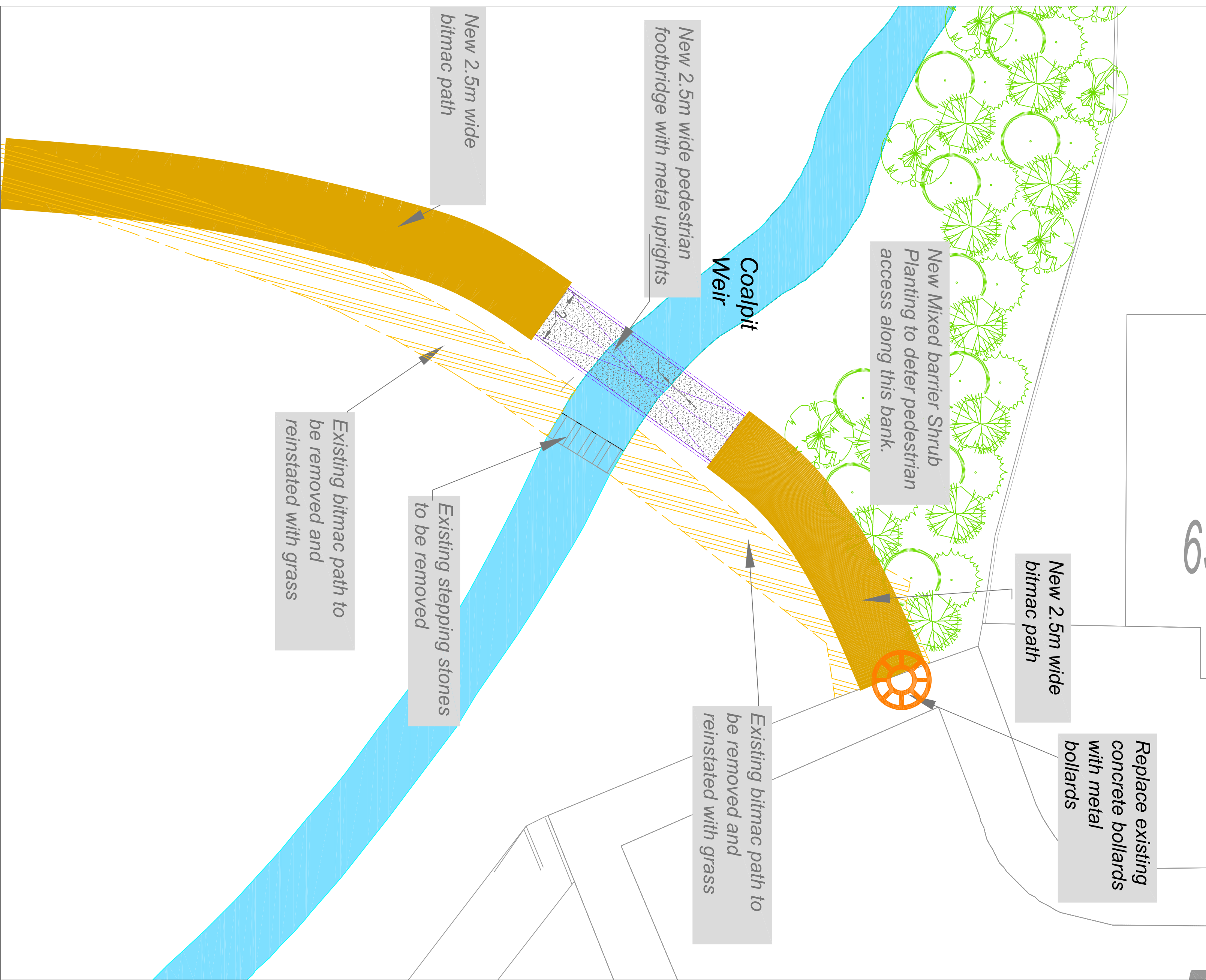
Example of proposed bridge
